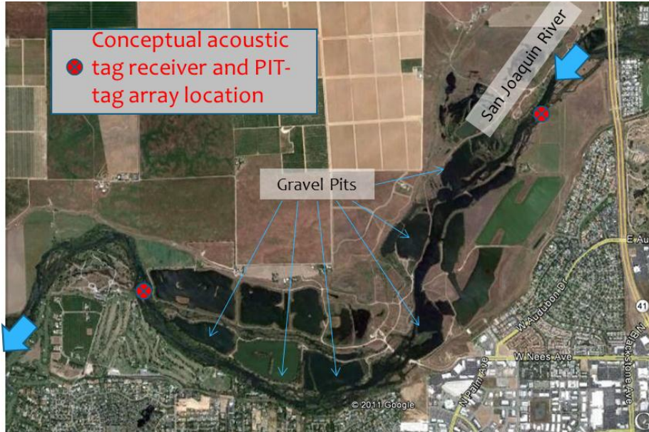
FIGURE 3: Conceptual placement of acoustic tag receivers to detect fish passage into and out of the gravel pit reach.
