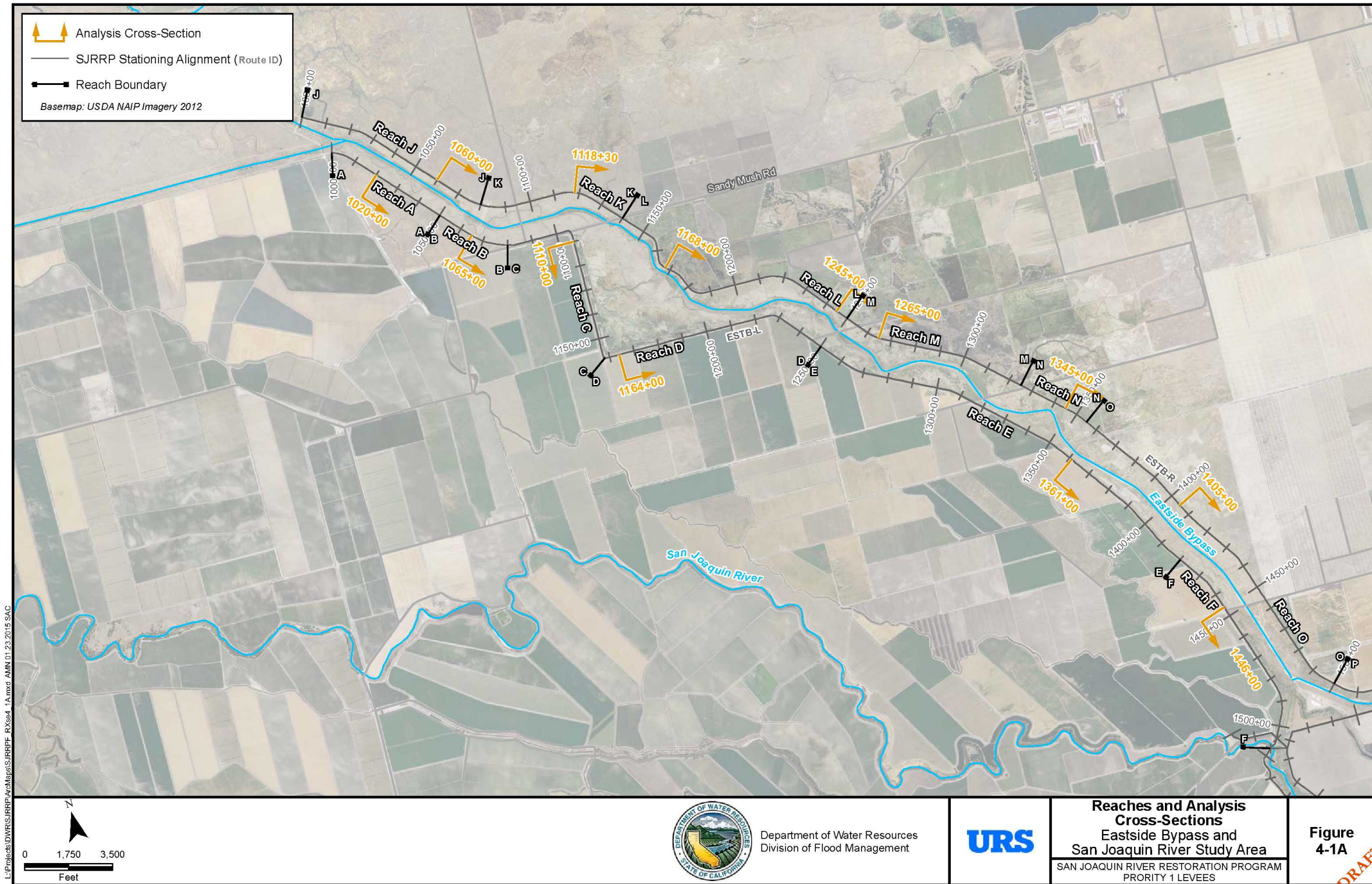
Figure 2. GCR analysis reaches and cross sections in the MESB (Figure 4-1a from URS, 2015).
