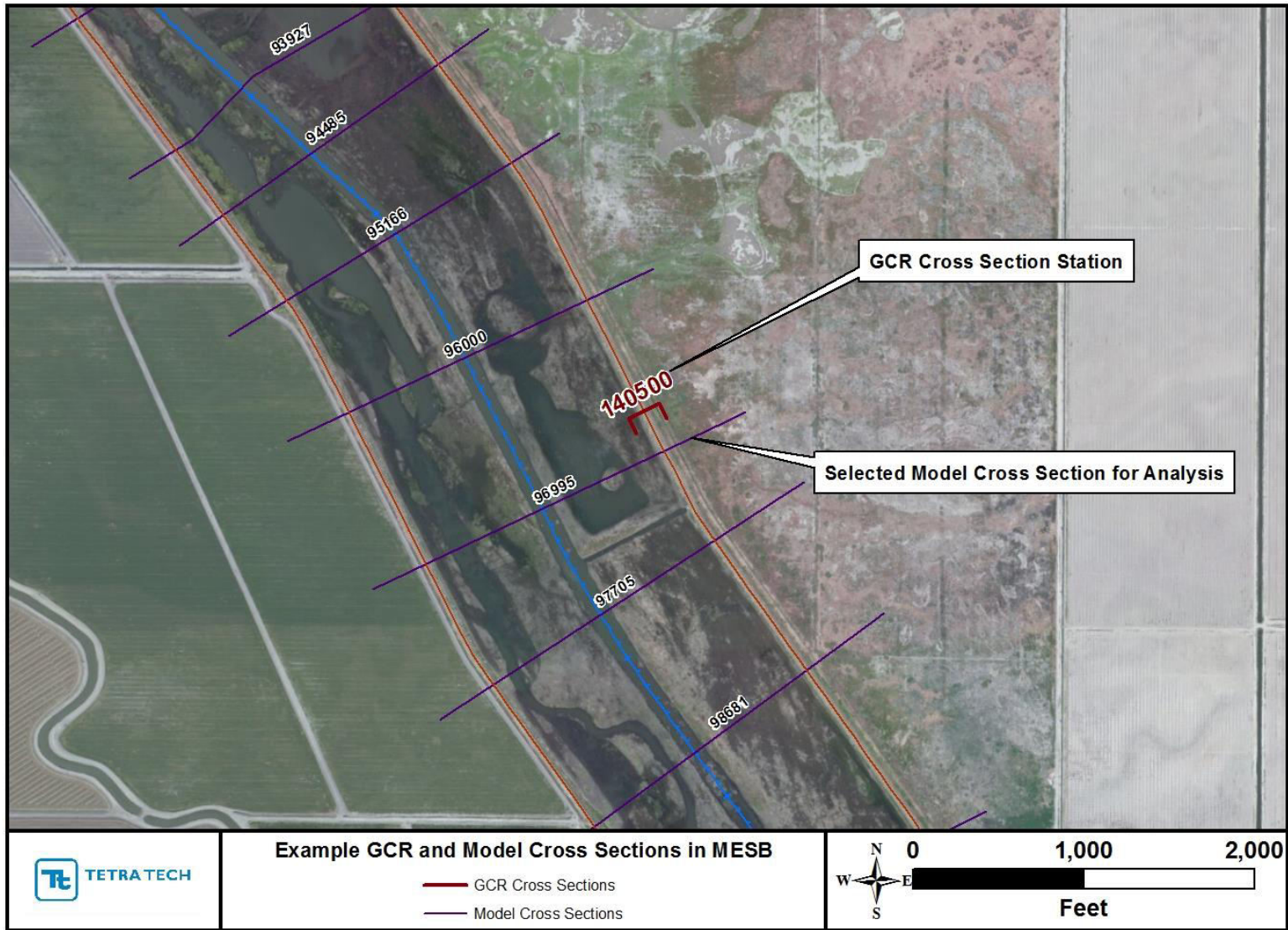
Figure 4. Planview of example GCR cross section and HEC-RAS model cross section selected for capacity calculations.
